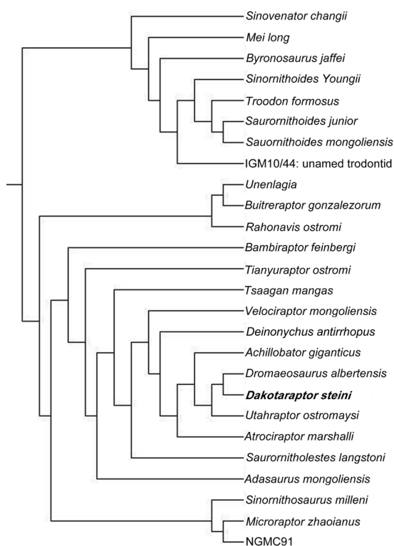
Figure 14. Phylogenetic relationships of Dakotaraptor steini within the Dromaeosauridae. Dakotaraptor is most closely allied with Dromaeosaurus albertensis , the most common dromaeosaurid in the Hell Creek Formation. The analysis was performed using a modified Theropod Working Group (TWiG) data set from Zheng and others, (2010).
