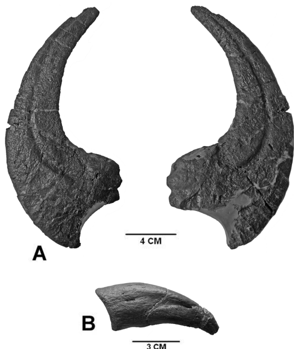
Figure 12. Pedal unguals from the Dakotaraptor holotype (PBMNH.P.10.113.T). A, the right raptorial pedal ungual II in lateral (left) and medial (right) views; B, right pedal ungual from digit III in lateral view. Note the bony tube that encloses the distal portion of the corial groove.
